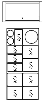
SINGLE DOOR OVEN, A STEAM TABLE THAT HOLDS (4)1/3 PANS, (6)1/2 PANS (1)SOUP POT AND (2)CONDIMENT POTS
